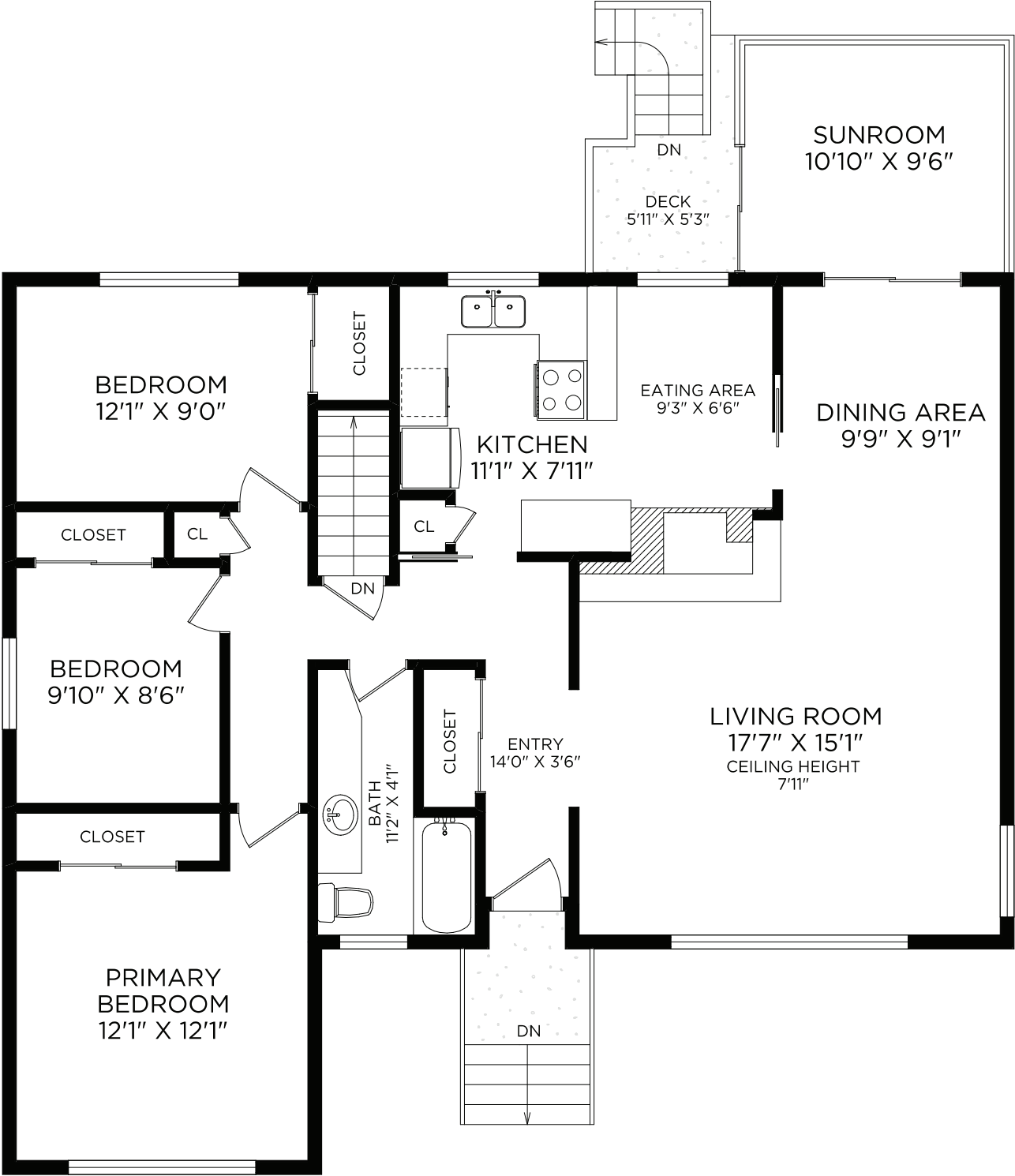
MAIN FLOOR
